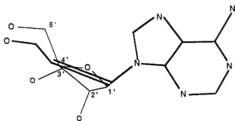
Figure 1. Computer-generated overlap of adenosine (3'-endo form) with ( S )-adenallene ( 3a ). Overlap was determined by using Computer Aided Molecular Modeling System (XICAMM), Xiris Corp., New Monmouth, NJ. Only the ribofuranose portion is numbered. All hydrogen atoms were omitted for clarity. Overlap of purine rings is virtually total. Cumulated system of double bonds of 3a is shown as a single double bond. Note proximity of \pi orbitals of allenic portion ( 3a ) with p orbitals of O_4' (adenosine) as well as that of O_3' (adenosine) and the corresponding oxygen atom of 3a . According to a referee, the distance between C-2' ( 3a ) and O-4' (adenosine) is 0.9 Å.
